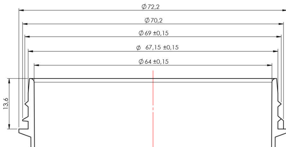
NECK DETAIL SCALE 2:1
